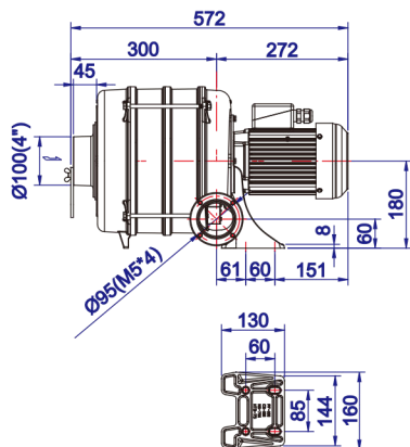
HTB75-104 4-stage
