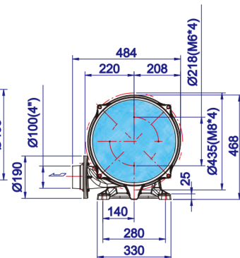
HTB100-505 5-stage
