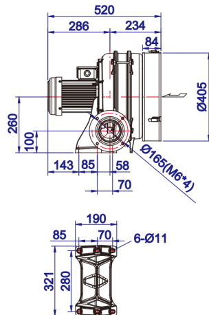
HTB100-203 3-stage
