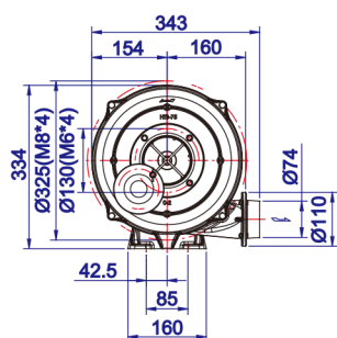
HTB75-105 5-stage
