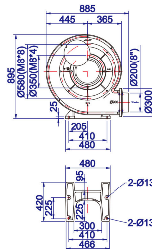
TB200-15 / TB200-20
