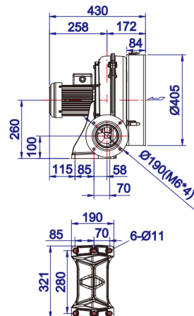
HTB100-102 2-stage
