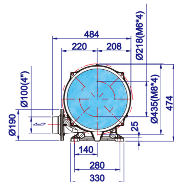
HTB100-102 2-stage
