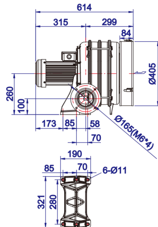
HTB100-304 4-stage
