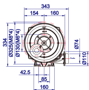
HTB75-053 3-stage
